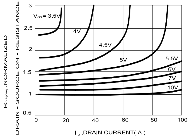
ON- RESISTANCE VARIATION WITH DRAIN CURRENT AND GATE
