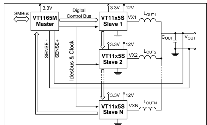
Figure 1. VT1165M System Architecture
